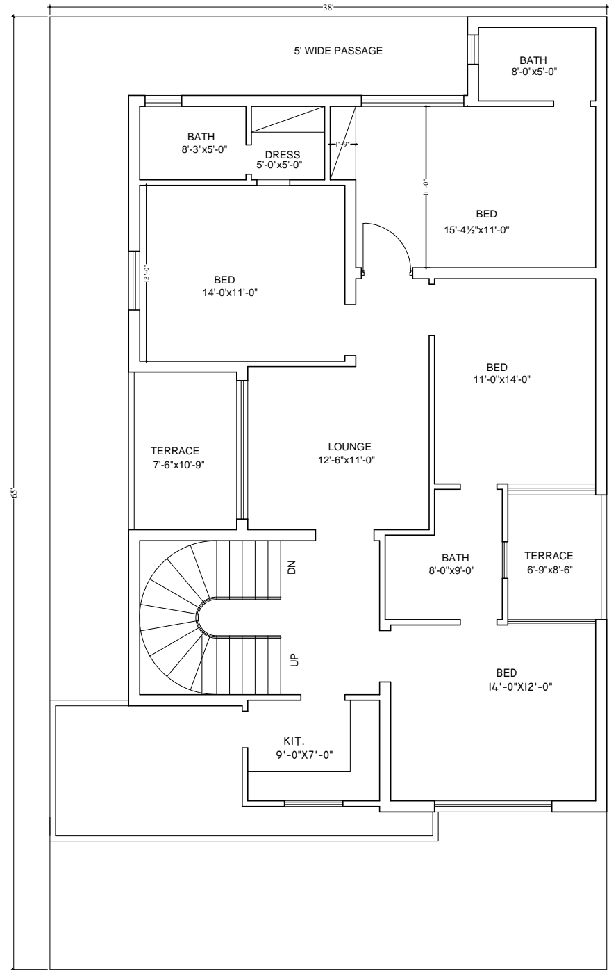
FIRST FLOOR
