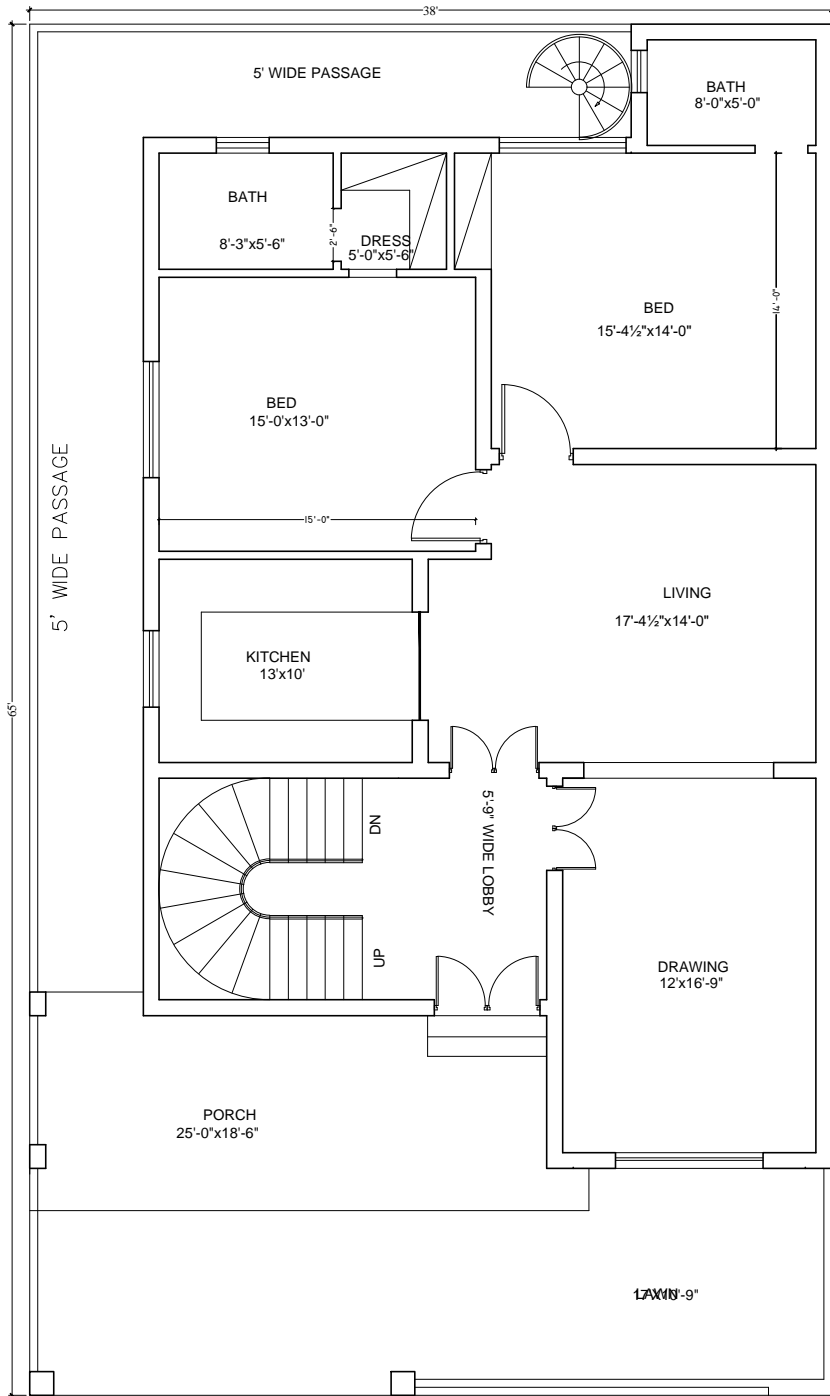
GROUND FLOOR
